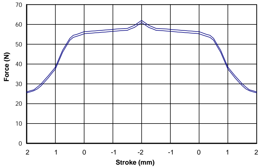
force stroke characteristic at 60% nominal current & 20°C with PWM
