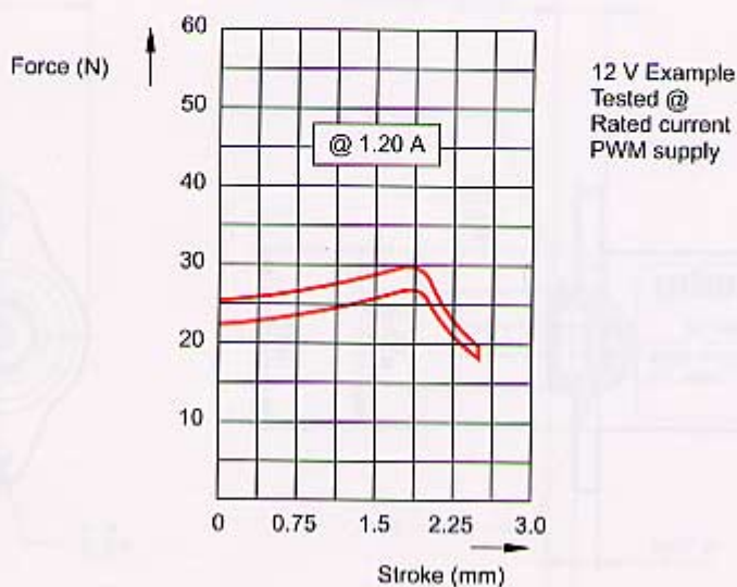
Force/Stroke Characteristic
