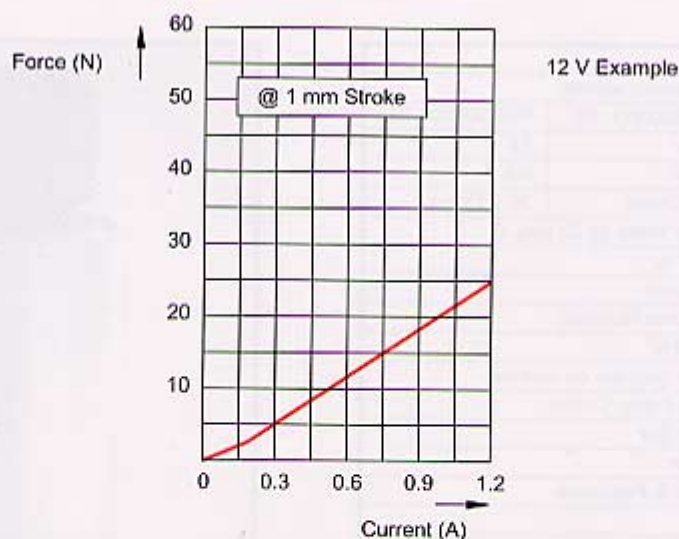
Force/Current Characteristic
