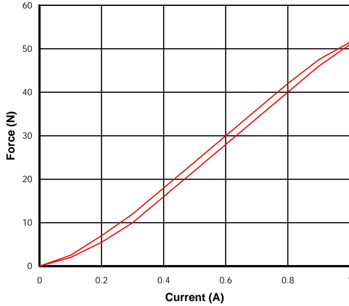
12V force current characteristic at 1mm stroke
