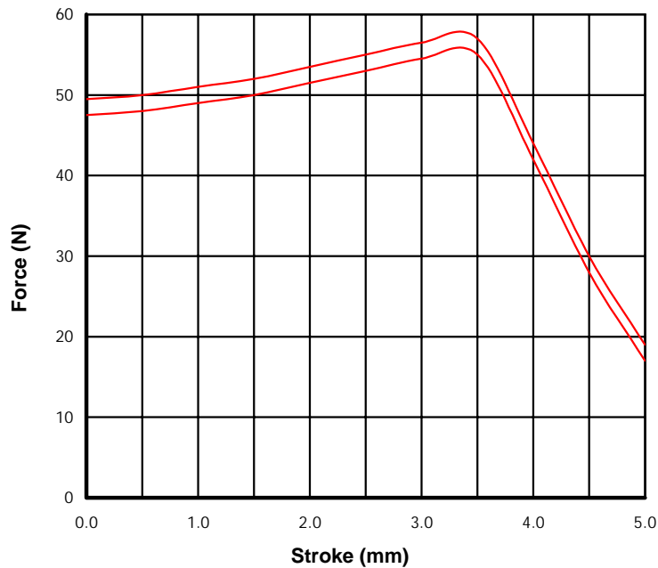
12V force stroke characteristic at nominal current, 20°C with PWM
